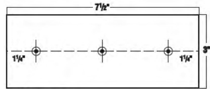
C-386 3" x 7 1/2" Base, Three Holes In Line, All Countersunk
