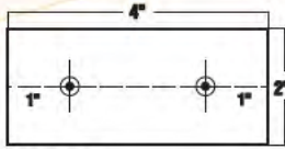
C-144 2" x 4" Two Holes Countersunk
