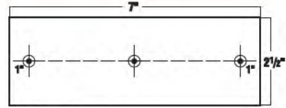
C-374 2 1/2" x 7" Lid, Three Holes In Line, All Countersunk
