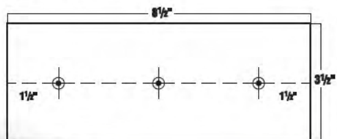
C-396 3 1/2" x 8 1/2" Base, Three Holes In Line, All Countersunk
