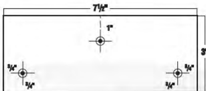
C-376 3" x 7 1/2" Three Holes Countersunk (Staggered)
