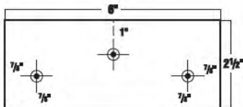
C-266 2 1/2" x 6" Three Holes Countersunk (Staggered)
