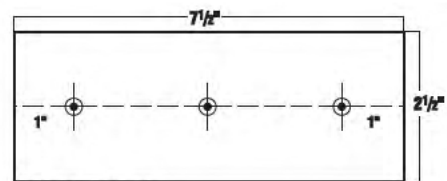
C-384 2 1/2" x 7 1/2" Lid, Three Holes In Line, All Countersunk
