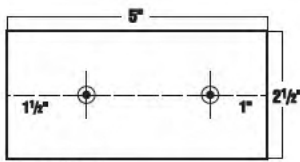
C-254 2 1/2" x 5" Two Holes Countersunk
